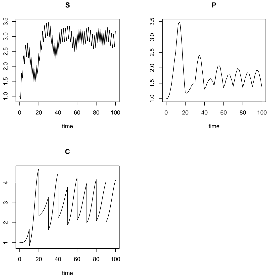
Figure 4: Solution of the Lotka-Volterra resource (S) – producer (P) – consumer (C) model with time-variable input (signal) and with half of the consumer removed every 10 days - see text for R-code
