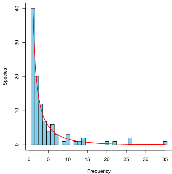
Figure 3: Fisher’s log-series fitted to one randomly selected site (25).
