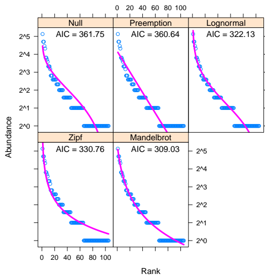
Figure 4: Ranked abundance distribution models for a random plot (no. 25). The best model has the lowest AIC.
